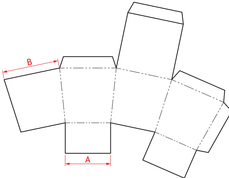
SURFACE DEVELOPMENT
