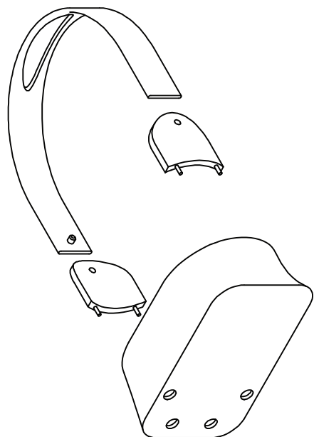
EXPLODED ISOMETRIC
