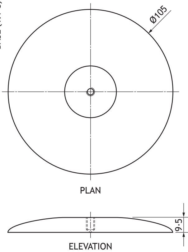
BASE (1:1.5)
