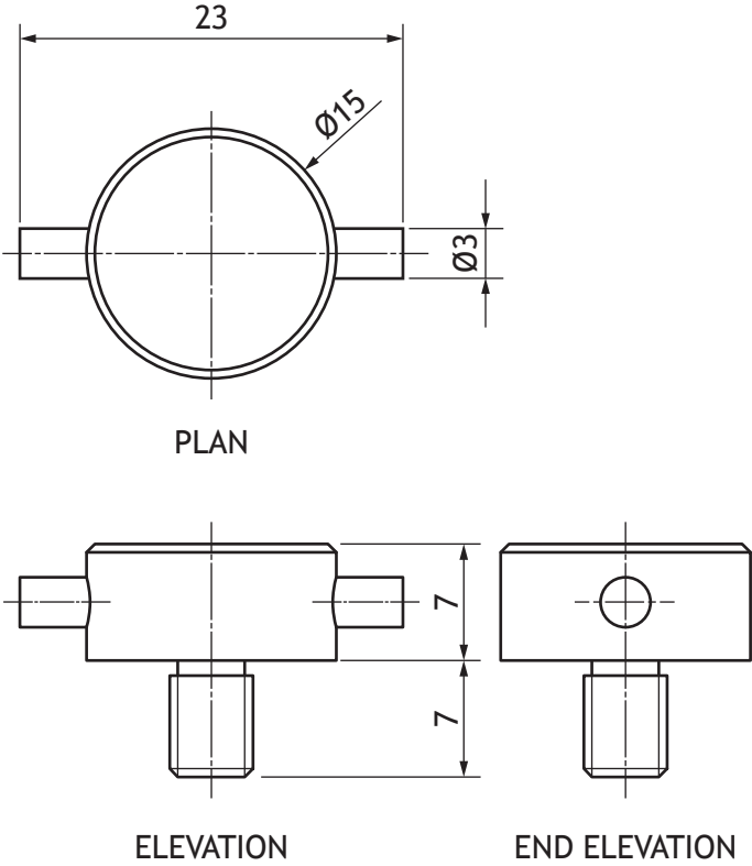
BASE (1:1.5)
