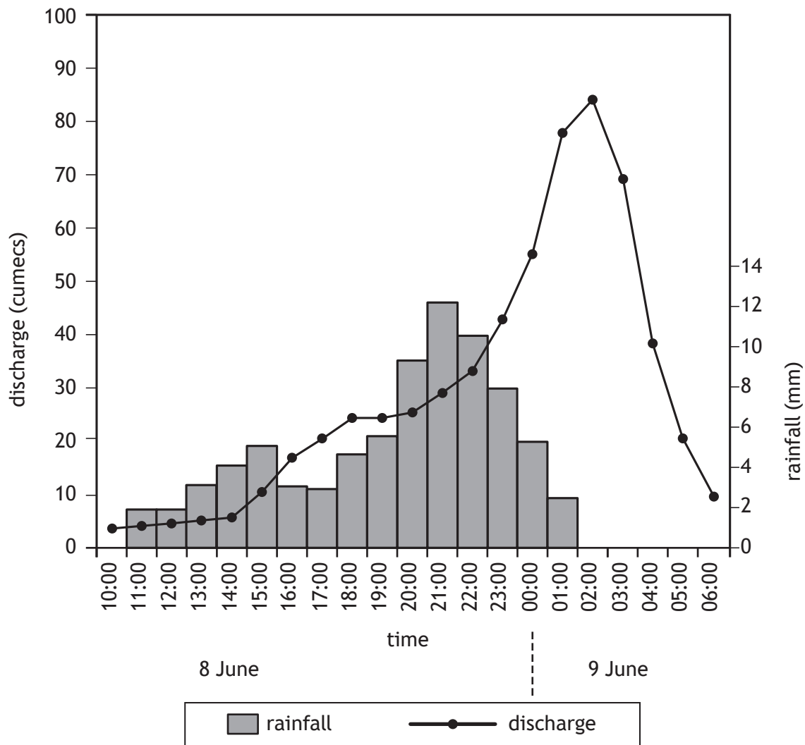
Diagram Q4 Flood hydrograph for the River Leri, West Wales, 8 th and 9 th June 2012
