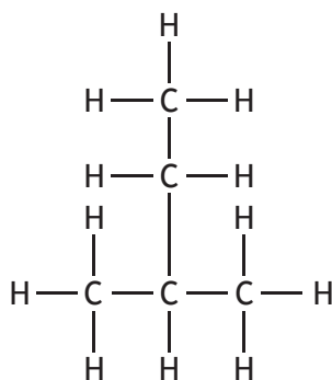
isopentane
